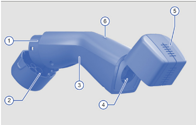
Fig. 1 Overview PowerSocket
